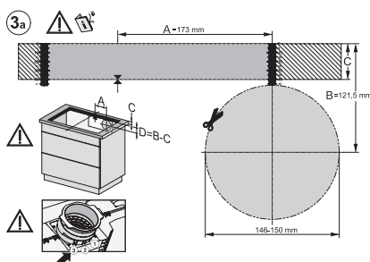
KMDA7272-1FL/FR, KMDA7473-1FL/FL MattFinish/FR, KMDA7272FL/FR, KMDA7473FL/FR – Installation variant 13 Circulating air
