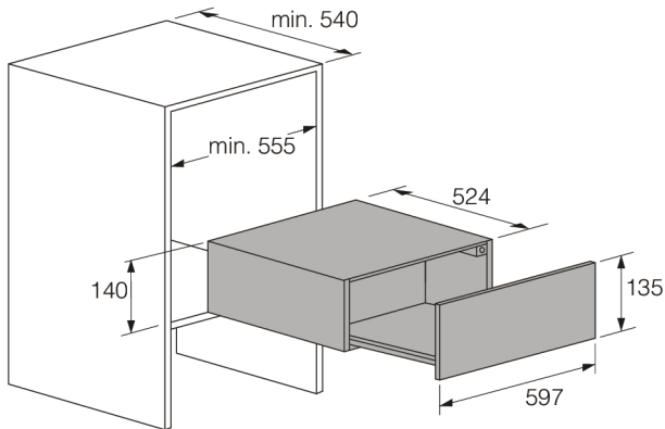
Craft warming drawer
