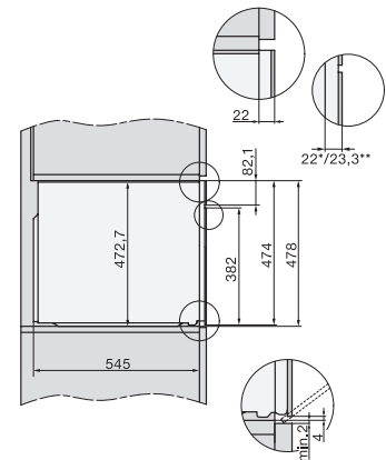
side view H7000 90 D1, installation drawings
