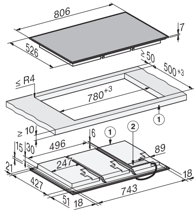
KM8684-2FR surface-mounted (*Fußnote) Installation drawing
